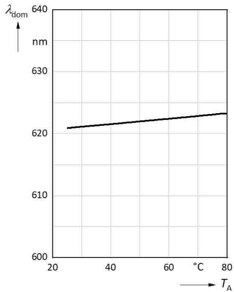
Dominant Wavelength vs. Ambiente Temperature
